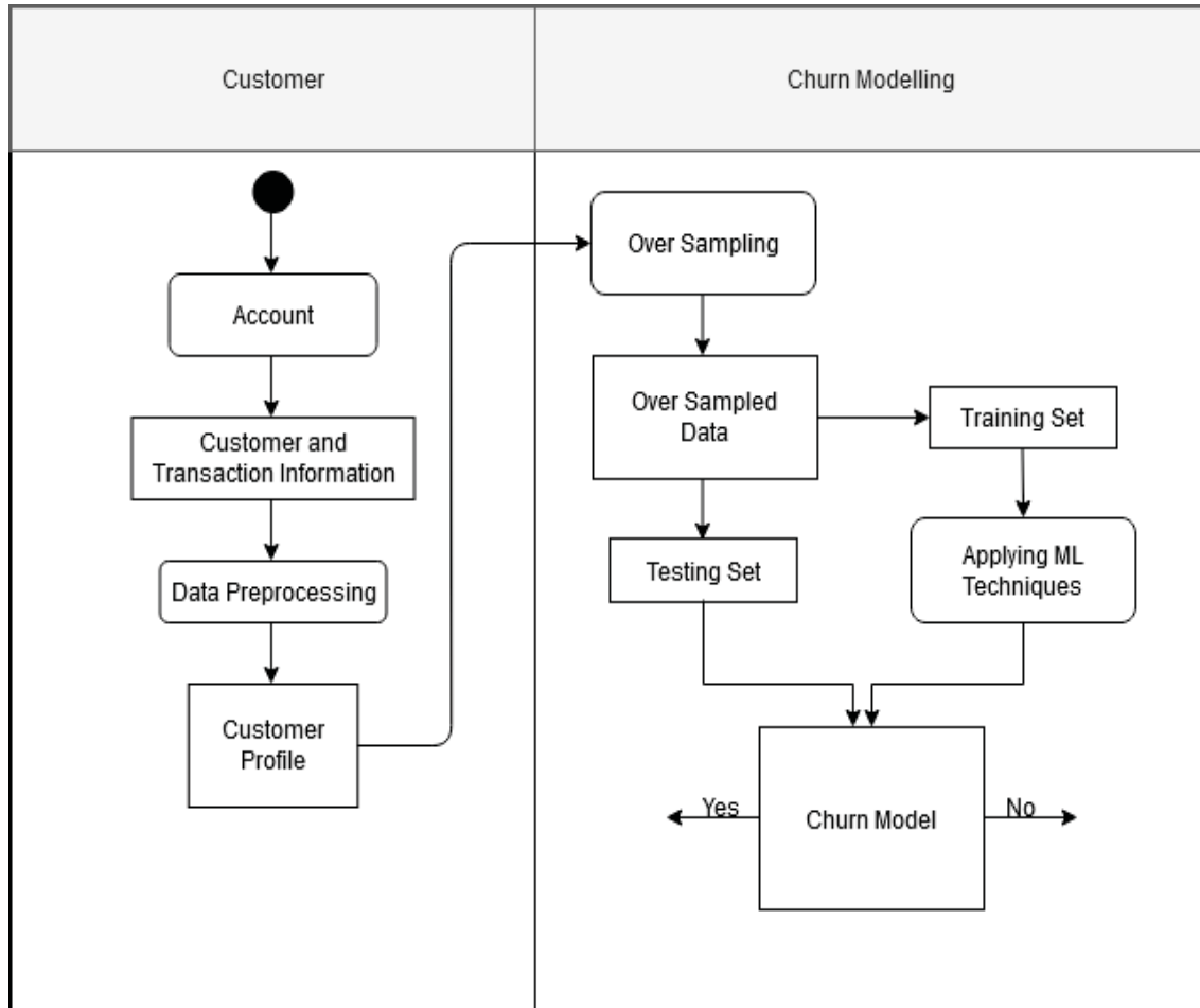
Fig.1. Activity diagram of the proposed system TABLE II
